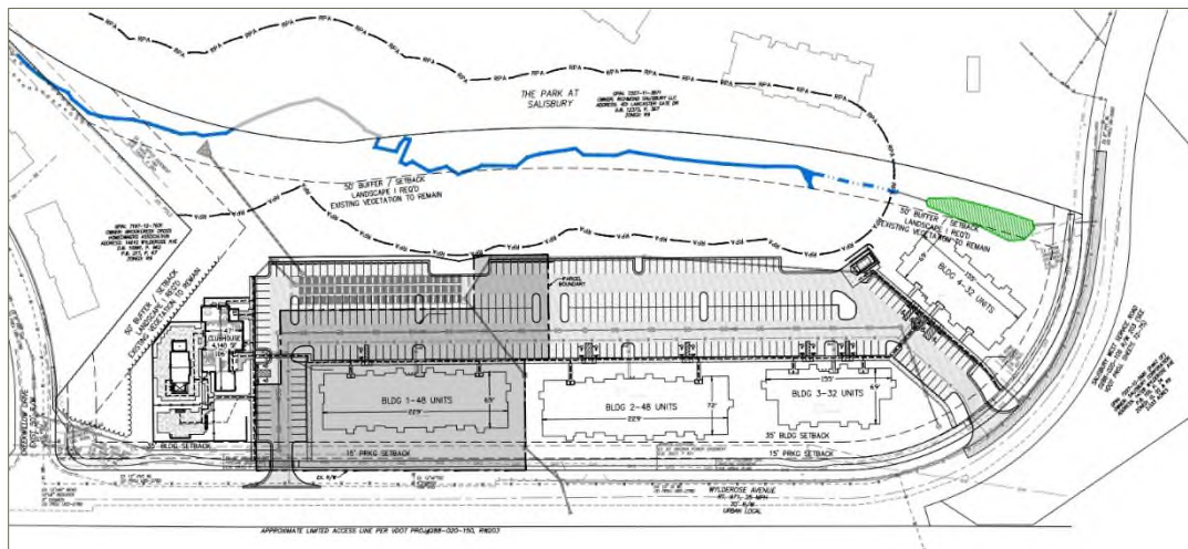
Figure 2 Site Plan, 288 Lofts
